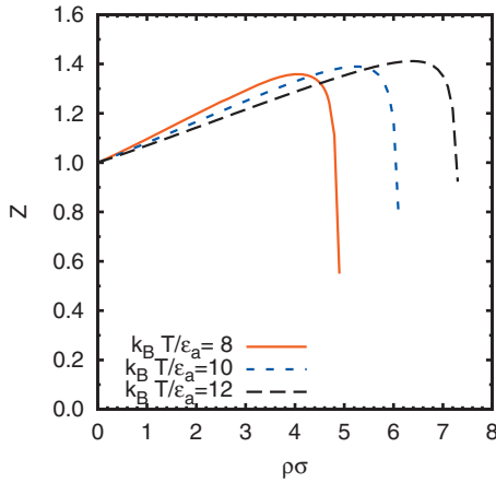
FIG. 1. Plot of the compressibility factor Z = \beta p / \rho as computed from the virial (-energy) route to the pressure for \epsilon_r / \epsilon_a = 2 and \Delta / \sigma = 1 . Results for three different reduced temperatures k_B T / \epsilon_a = 8, 10, 12 are displayed.
