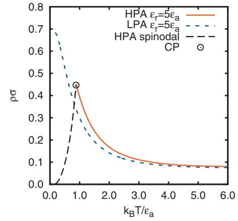
FIG. 9. Plot of the FW transition line in the \rho\sigma vs k_B T / \epsilon_a plane with \Delta / \sigma = 1 and \epsilon_r / \epsilon_a = 10 (top panel) and \epsilon_r / \epsilon_a = 5 (bottom panel). The long dashed curves are the spinodal lines predicted by the HPA. The FW and spinodal lines meet at the critical point (denoted by a circle).
