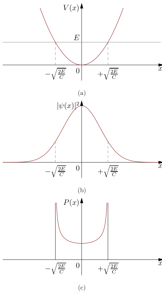
FIG. 1.5. Comparison between (c) classical and (b) quantum probability densities for an harmonic oscillator whose potential is shown in (a).
