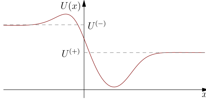
FIG. 1.3. Potential U(x) and its asymptotic behavior at \pm\infty .
