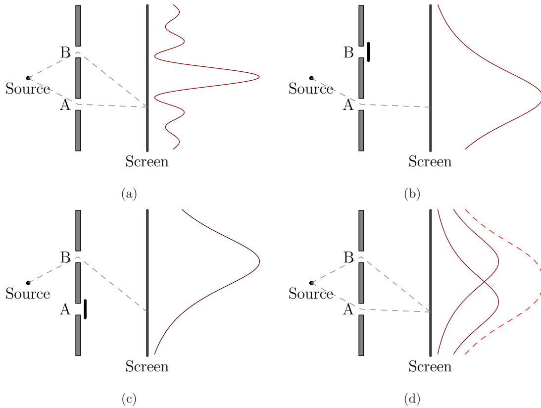
FIG. 13.2. (a) The probability P_{AB} with both slits open. (b) The probability P_A obtained keeping open the slit A (c) The probability P_B obtained keeping open the slit B (d) The probability P_A + P_B . We see that P_{AB} \neq P_A + P_B .
