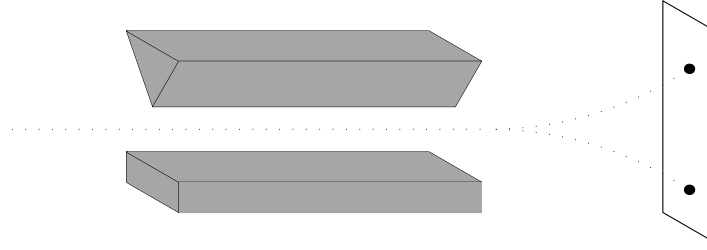
FIG. 7.1. Illustration of the Stern-Gerlach experiment.
