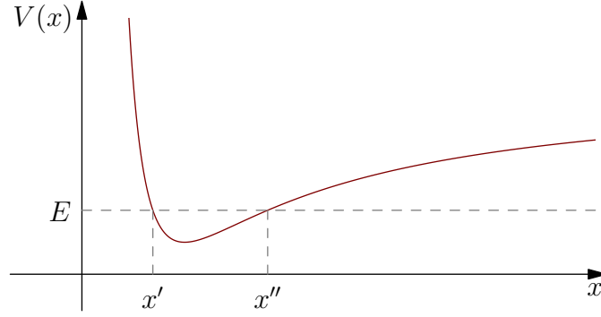
FIG. 1.1. The potential V(x) used in the qualitative analysis of the stationary Schrödinger equation and the energy E chosen for the analysis.
