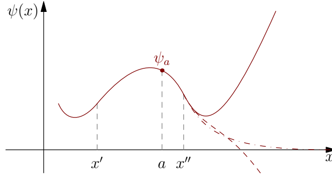
FIG. 1.2. Three attempts to find an acceptable solution to the time-independent Schrödinger equation.
