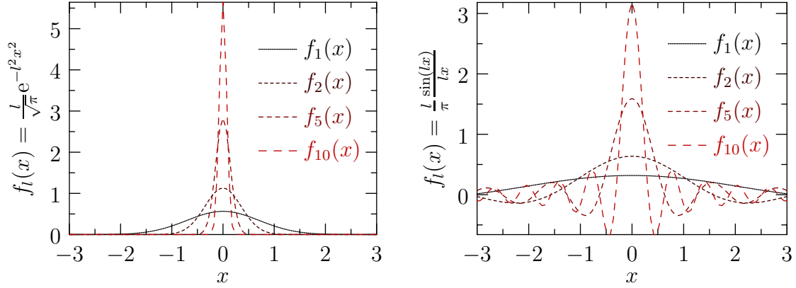
FIG. 1.4. Representations of the Dirac delta \delta(x) .
