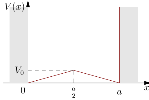
FIG. 10.2. Infinite well with a perturbation
