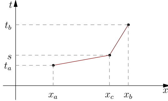
FIG. 13.5. Schematic representation of F(s) .
