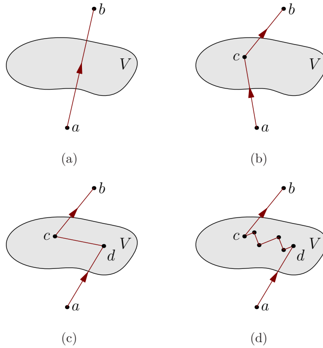
FIG. 13.6. Schematic representation of series expansion Eqn. (13.23).
