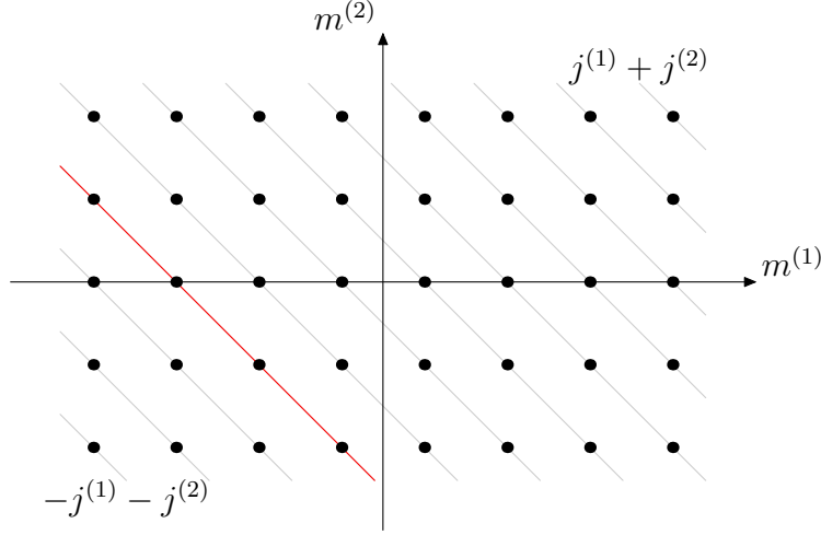
FIG. 5.2. Addition of angular momenta. The bullets display all the pairs (m^{(1)}, m^{(2)}) for j^{(1)} = 7/2 and j^{(2)} = 2 . Remember that the only allowed values of m^{(1)} and m^{(2)} given j^{(1)} and j^{(2)} are m^{(1,2)} = -j^{(1,2)}, -j^{(1,2)} + 1, \dots, j^{(1,2)} - 1, j^{(1,2)} thus m^{(1)} = -7/2, -5/2, \dots, 5/2, 7/2 and m^{(2)} = -2, -1, 0, 1, 2 . The lines correspond to M^{(T)} = m^{(1)} + m^{(2)} . For example, the red line in figure is the line of the pairs (m^{(1)}, m^{(2)}) such that M^{(T)} = -j^{(1)} - j^{(2)} + 3 . To count the number of pairs n(M^{(T)}) you have simply to count how many pairs are situated along the line corresponding to M^{(T)} .
