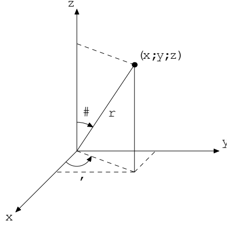
FIG. 5.1. Polar coordinates.
