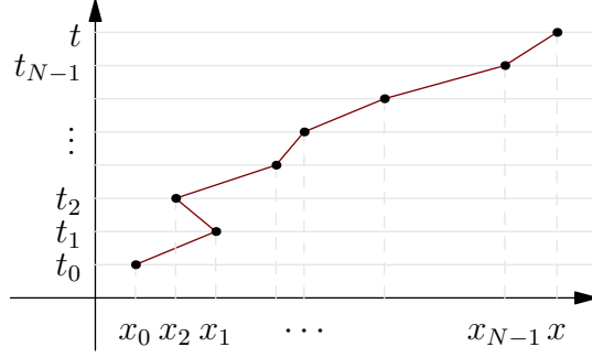
FIG. 13.4. The discretized approximation of the path integral
