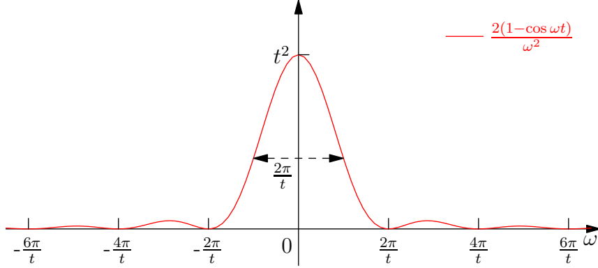
FIG. 12.2. Plot of f(t, \omega) .
