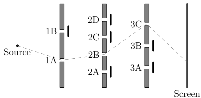
FIG. 13.3. More screens with different openings.
