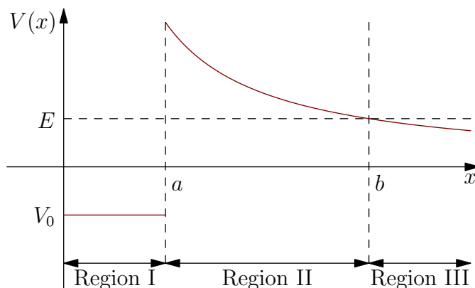
FIG. 14.1. Model of potential barrier in the \alpha decay of the nuclei.
