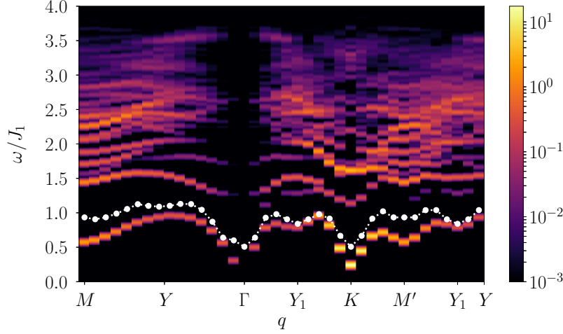
Figure 4.20: The same as Fig. 4.19 but for the optimal variational wave function with both hopping t and fictitious magnetic field h . The path along the Brillouin zone is shown in Fig. 4.18. The dotted line denotes the bottom of the continuum E_q = \min_k \{E_0^{q-k} + E_0^k\} , where E_0^q is the lowest energy for a given momentum q obtained within our variational approach. Since the spectrum is gapless at the \Gamma point, we exclude the cases k = (0, 0) and k = q in the search of the minimum, because the resulting E_q would simply coincide with the energy of the magnon branch E_0^q all over the Brillouin zone. The purpose of this kinematic analysis is to show that no magnon decay can yield an energy E_q which is lower than the one of the magnon branch E_0^q (in contrast with spin wave results).
