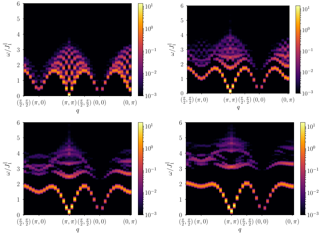
Figure 4.9: Dynamical spin structure factor of the spatially anisotropic Heisenberg model of coupled chains (4.8). Different values of the inter-chain couplings are reported: J_1^\perp/J_1^\parallel = 0.1 (upper left), 0.3 (upper right), 0.5 (lower left), and 0.7 (lower right). The square cluster contains N = 22 \times 22 sites. Spectral functions have been convoluted with normalized Gaussians with standard deviation 0.05J_1^\parallel .
