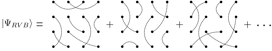
Figure 1.3: Schematic representations of RVB spin liquids. For the sake of simplicity, the expansion coefficients \phi(C) of the linear combination (1.3) are not explicitly shown in the picture.
