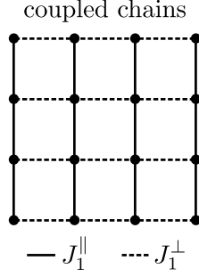
Figure 4.8: Exchange couplings of the anisotropic Heisenberg model of Eq. (4.8).
